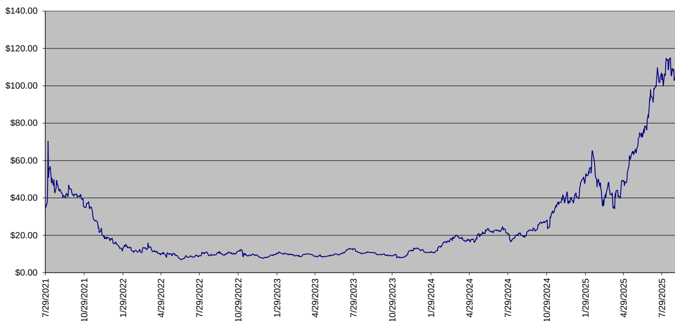
Underlier Daily Closing Levels July 29, 2021* to September 8, 2025
